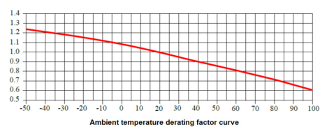
Ambient temperature derating factor curve
