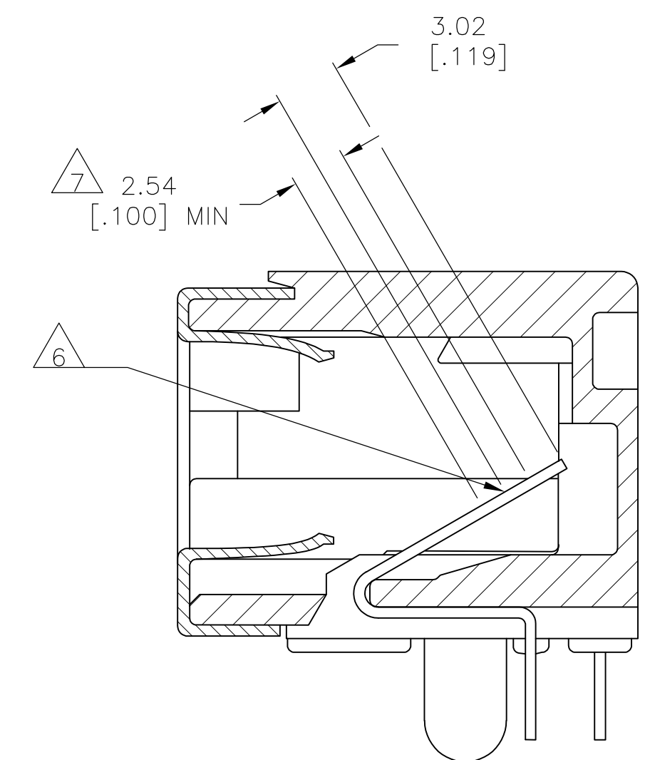
SECTION J-J
